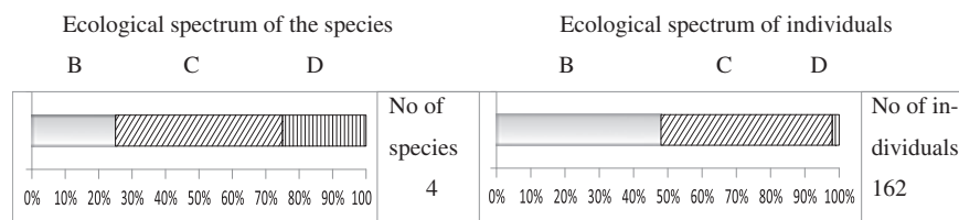
Fig. 25. Ecological structure of malacocenosis from cultural layer of site Valea Morilor.
